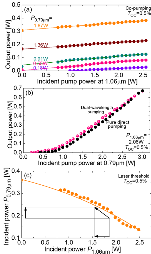
Fig. 7. 2.3 μm Tm laser with a cross-polarization dual-wavelength pumping at 0.79 μm and 1.06 μm (the ^3\text{H}_6 \rightarrow ^3\text{H}_4 GSA and ^3\text{F}_4 \rightarrow ^3\text{F}_{2,3} ESA transitions): (a) output power vs. the incident pump power at 1.06 μm for fixed seeding pump powers at 0.79 μm; (b) input-output dependences for T_{OC} = 0.5\% : pure and dual-wavelength pumping; (c) laser threshold as a function of the incident pump power at both pump wavelengths, T_{OC} = 0.5\% .
