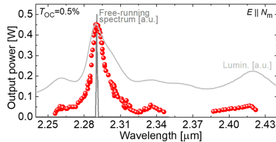
Fig. 10. Wavelength tuning curve for a Tm laser operating on the {}^3\text{H}_4 \rightarrow {}^3\text{H}_5 transition with a pure direct pumping at 0.79 \mu\text{m} , light grey curve – luminescence spectrum, dark grey curve – free-running laser spectrum, P_{0.79\mu\text{m}} = 2.9 \text{ W} , T_{\text{OC}} = 0.5\% , laser polarization: E \parallel N_m .
