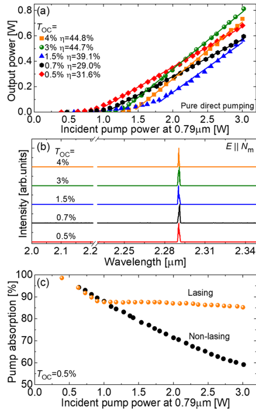
Fig. 6. 2.3 μm Tm laser with a pure direct pumping at 0.79 μm (the ^3\text{H}_6 \rightarrow ^3\text{H}_4 GSA transition): (a) input-output dependences, \eta – slope efficiency; (b) typical spectra of laser emission measured well above the laser threshold, laser polarization: E \parallel N_m ; (c) total (double-pass) pump absorption under non-lasing and lasing (for T_{OC} = 0.5\% ) conditions.
