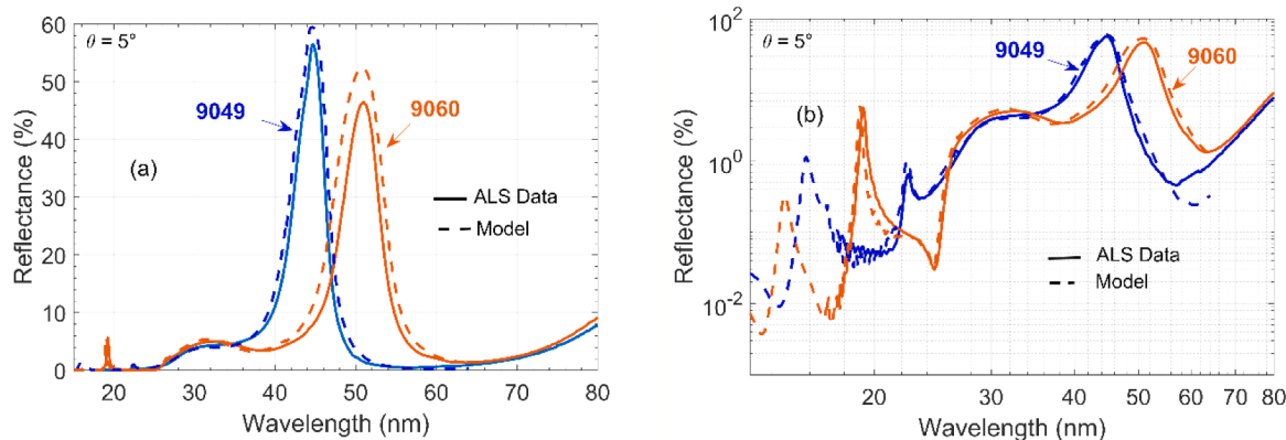
Fig. 12. Measured (solid line) and fitted (dash line) reflectance vs. wavelength values for optimized Al/Sc/SiC multilayers in the EUV in linear scale (a) and logarithmic scale (b). (For interpretation of the references to color in this figure legend, the reader is referred to the web version of this article.)
