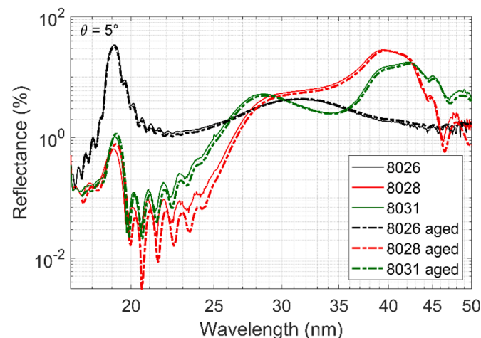
Fig. 9. Reflectance vs. wavelength measurements (plotted in log-log axes) of 8026, 8028 and 8031 Al/Sc multilayer samples in November 2018 and in August 2019.
