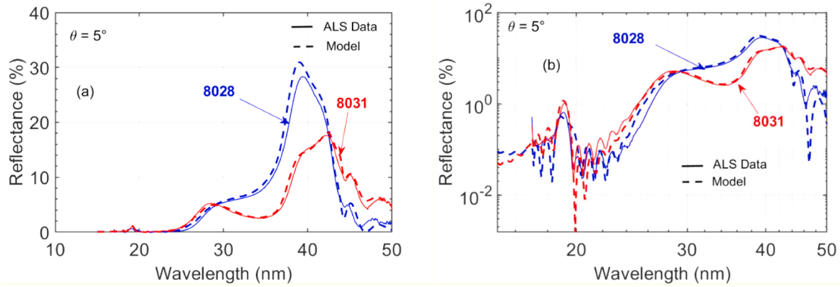
Fig. 6. Measured and fitted reflectance vs. wavelength data for the 8028 (Al/Sc) and 8031 (Sc/Al) samples near normal incidence ( \theta = 5^\circ ) in linear (a) and logarithmic scale (b). The 2 nd order multilayer Bragg peak is visible near 19 nm wavelength, in (b).
