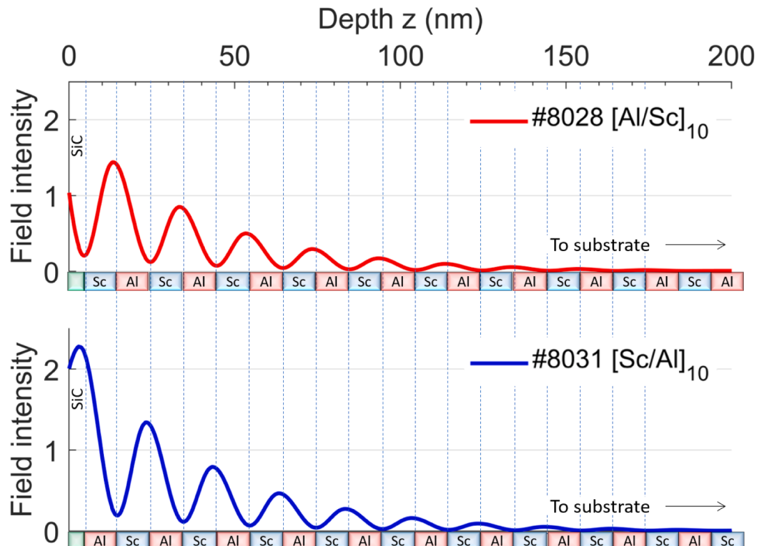
Fig. 7. Effect of deposition order and top (capping) layer on the intensity of the electric field in [Al/Sc] 10 8028 and [Sc/Al] 10 8031 multilayer coatings.
