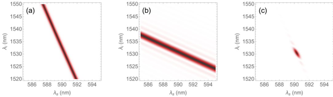
Figure 5: Example of a plot of |g(\omega_p, \omega_s, \omega_I)|^2 (a), of |f(\omega_p, \omega_s, \omega_I)|^2 (b), and of their product (c) giving JSA(\omega_p, \omega_s, \omega_I) = |JSA(\omega_p, \omega_s, \omega_I)|^2 for a given pump wavelength. The calculation uses the typical parameters of the experiment.
