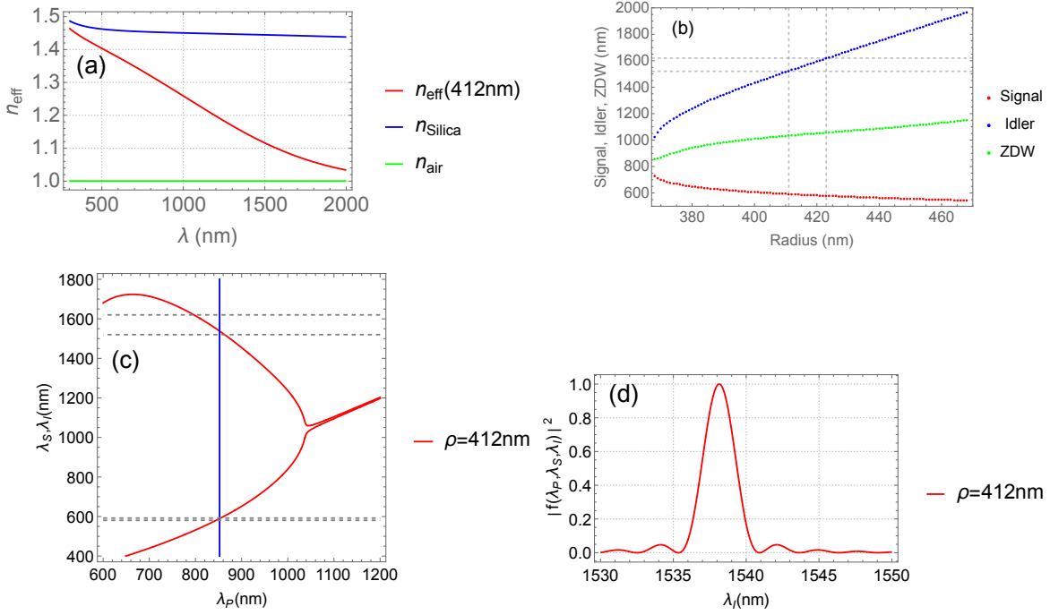
Figure 6: (a) Simulated value of the fundamental HE11 mode effective index for a nanofiber radius of 412nm. n_{\text{eff}} varies from the silica refractive index at wavelength where the mode is highly confined in the nanofiber core, to the air refractive index when the mode is deconfined. (b) From the effective index we can calculate the Zero Dispersion wavelength as a function of the nanofiber radius (green/light gray curve) and by solving the energy ( \omega_{S0} - \omega_{I0} - 2\omega_{P0} = 0 ) and momentum ( 2\beta(\omega_{P0}) - \beta(\omega_{S0}) - \beta(\omega_{I0}) = 0 ) conservation equation simultaneously we can calculate for each radius the emitted Signal (red/red gray curve) and Idler (blue/dark gray curve) wavelength values as a function of radius for a pump wavelength of 852,2nm. This allows to determine the radius range allowing emission of idler photons in the telecom band (gray dashed lines). (c) the same calculation can also be performed for a fixed radius (here 412nm) as a function of pump wavelength, to evaluate tolerance on pump wavelength. (d) Finally, we can calculate the shape of emission spectra by tracing \text{Sinc}^2[(2\beta(\omega_{P0}) - \beta(\omega_S) - \beta(\omega_I))L/2] for a nanofiber of length L=1\text{cm} at energy conservation.
