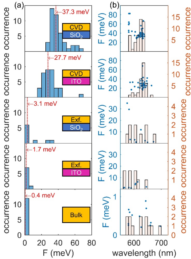
Figure 4. Effect of hBN crystal and substrate type on inhomogeneous broadening. Panel (a) is a histogram of linewidths for emitters and panel (b) is the scatter plot of linewidth against the ZPL wavelength and histogram of the number of occurrences of a ZPL wavelength, from top to bottom this figure shows the result for CVD film on SiO 2 substrate, CVD film on ITO substrate, exfoliated flake on SiO 2 substrate, exfoliated flake on ITO substrate, and bulk hBN crystal respectively. The red dashed line shows the median of inhomogeneous linewidth for each sample.
