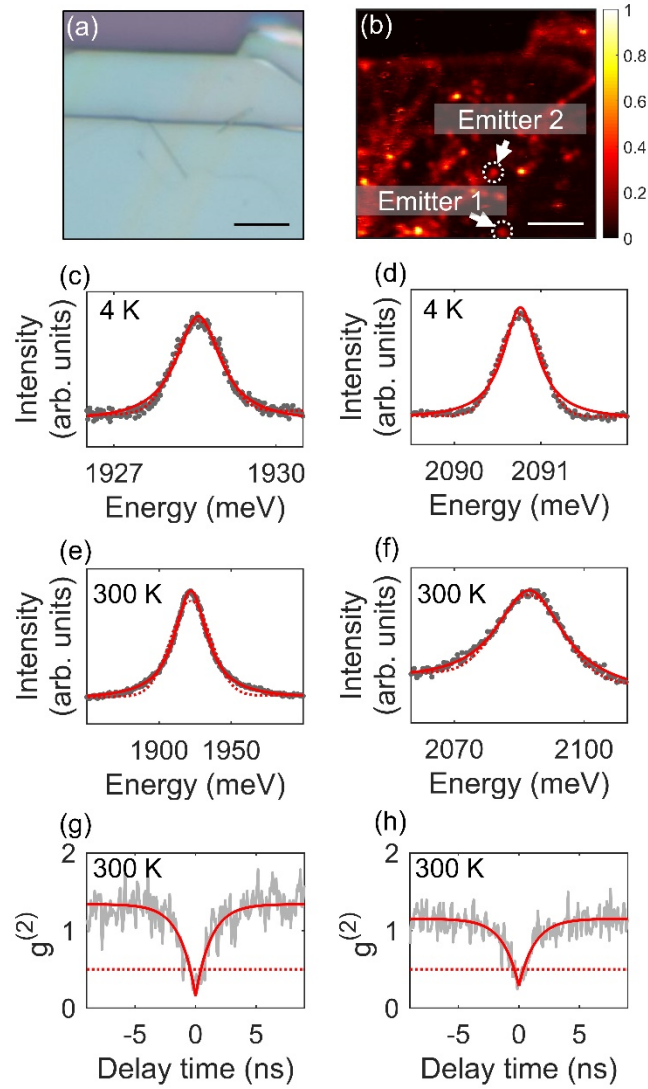
Figure 2. Quantum emitters in bulk hBN. (a) Microscope image and (b) photoluminescence map of a bulk hBN crystal. The arrows show the position of two emitters under study; scale bar corresponds to 5 \mu\text{m} . (c) 4 K and (e) 300 K spectra of ZPL of emitter 1. Solid line shows Lorentzian and the dashed line shows Gaussian fits (g) shows photon anti-bunching for emitter 1. (d), (f), and (h) show the same plots for emitter 2.
