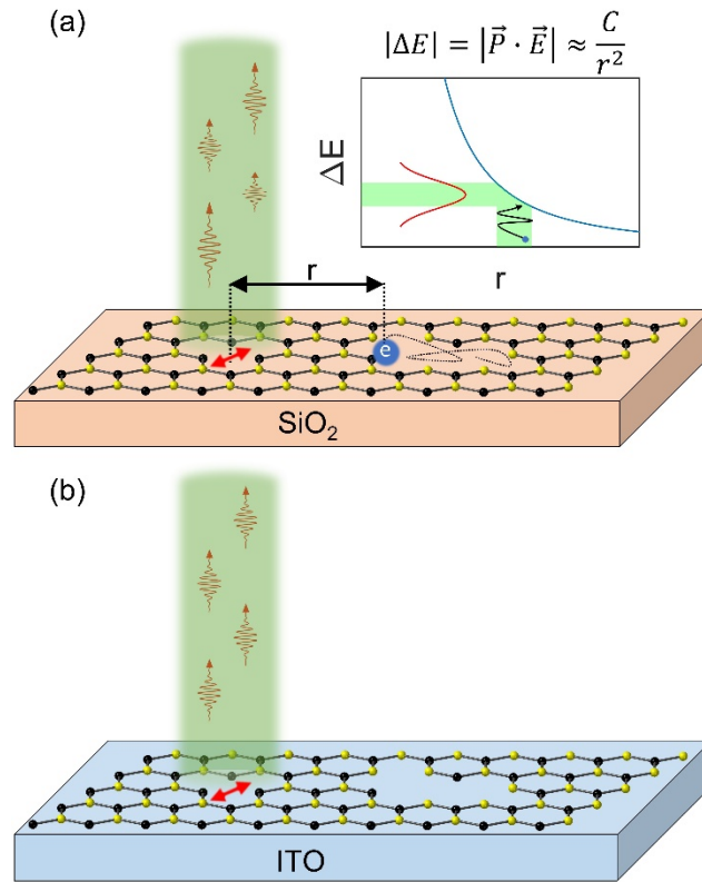
Figure 1. Schematic of substrate effect on spectral diffusion of single photon emitters in hBN. (a) hBN emitter on an insulating SiO 2 substrate is prone to larger spectral diffusion due to charge traps in hBN, SiO 2 , and their interface. The inset shows Stark shift dependence on distance of nearby charges and how changes in the local charge distribution can broaden the linewidth. (b) hBN emitter on an ITO substrate shows narrower linewidth as a result of fewer charge traps in hBN, ITO, and their interface.
