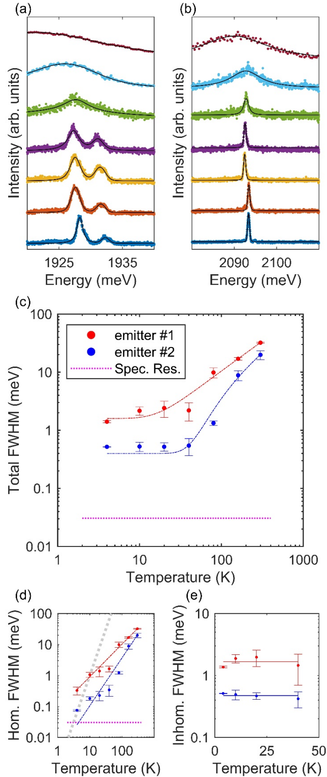
Figure 3. Temperature dependence of ZPL for emitters in bulk hBN. Effect of temperature on lineshape for emitter 1 (a) and emitter 2 (b) from 4 K to 300 K. (c) Linewidth against temperature for two emitters under study. Linear fits for temperatures below and above 40 K are shown; dashed lines are fits with a model equation (4), and the dashed magenta line shows the spectral resolution of the spectrometer used in this study. In (d) and (e) homogeneous and inhomogeneous components of linewidth extracted by Voigt fit are plotted as a function of temperature. The slope of
