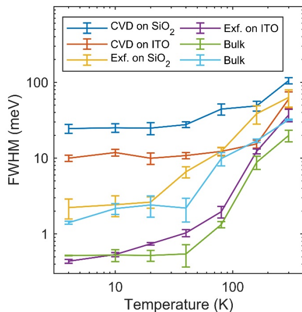
Figure 5. Temperature dependence of ZPL FWHM for various emitters in bulk hBN, 5 nm thick exfoliated hBN on SiO 2 , 8 nm thick exfoliated hBN on ITO, 5 nm thick CVD hBN on SiO 2 , and 5 nm thick CVD hBN on ITO. The result illustrates the total FWHM for temperatures from 4 K to 300 K.
