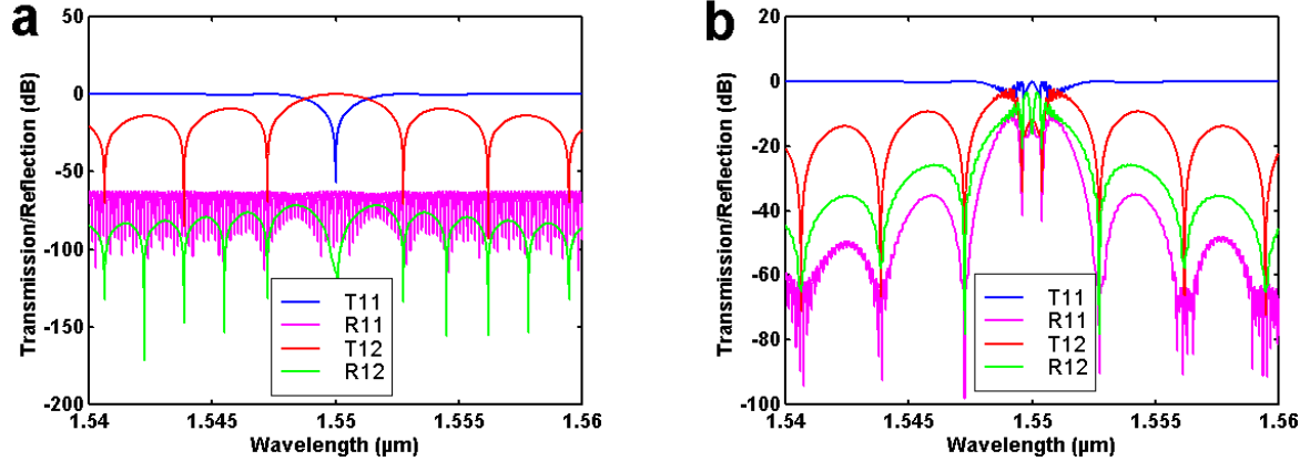
Figure 5. Spectral response of a PT-SBG assisted directional coupler with rectangular grating profile. Gain and loss grating sections are indicated by red and blue colors, respectively: a) Symmetric gain/loss index profile distribution between top and bottom waveguides; b) Anti-symmetric gain/loss index profile distribution between top and bottom waveguides.
