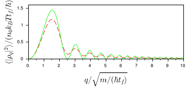
FIG. 4. Density ripples power spectrum for a homogeneous gas. The exact formula Eq. (B3) (dashed curve) is compared to the small q approximation given Eq. (5) of the main text, where \langle |\rho(q)|^2 \rangle is proportional to \langle \theta_q^2 \rangle (solid curve). The only relevant parameter is \hbar t_f / (m l_c^2) . Results are shown for \hbar t_f / (m l_c^2) = 0.05 , a value corresponding to the data depicted in Fig. (2,b) of the main text, the correlation length l_c = 2\hbar^2 n_0 / (m k_B T) being computed for the central density. The effect of the imaging resolution is to multiply this theoretical power spectrum with e^{-\sigma^2 q^2} , where \sigma is the rms width of the imaging pulse response function, assumed to be Gaussian. For our data, \sigma \sqrt{m / (\hbar t_f)} = 0.85 and only the first maximum of \langle |\rho(q)|^2 \rangle remains visible.
