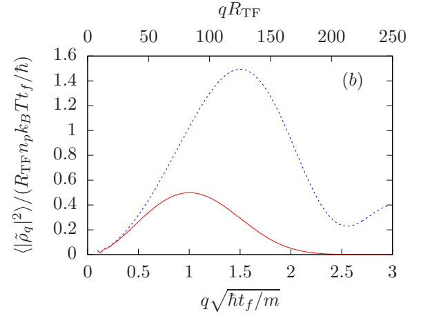
FIG. 7. Effect of the finite resolution (color online). We consider a cloud at thermal equilibrium in a harmonic potential with the same parameters as in Fig. 6. The power spectrum for infinite resolution (blue dashed curve) is compared to the power spectrum expected for a finite imaging resolution (red solid curve). The effect of the imaging resolution is to multiply the power spectrum with e^{-\sigma^2 q^2} , where \sigma is the rms width of the imaging pulse response function, assumed to be Gaussian. Here we took \sigma\sqrt{m/(\hbar t_f)} = 0.85 , a value close to that of experimental data.
