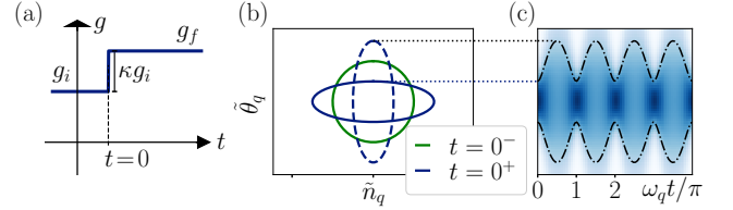
FIG. 1. Squeezing of each collective mode after an interaction strength quench. The Gaussian space distributions before the quench (green circle), just after the quench (solid ellipse) and after an evolution time \pi/(2\omega_q) (dashed ellipse) are represented in (b), where lines correspond to a given probability density. The subsequent breathing is seen in (c), where the time evolution of the phase distribution is shown.
