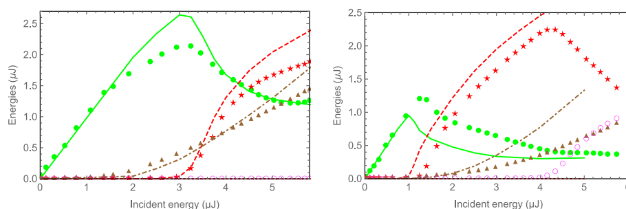
Fig. 7 Experimentally measured output energies versus the incident pump energy. The green disks correspond to the transmitted pump, the red stars correspond to the forward Raman and the brown triangles correspond to the reflected Brillouin. The lines correspond to the simulations (see text). Left figure is for a fiber length of L = 0.5 \text{ m} and the right one is for L = 1.5 \text{ m}
