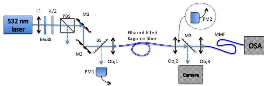
Fig. 6 Sketch of the experimental set-up, details are in the text
