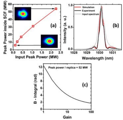
Fig. 5. (a) Output peak power per pulse versus input peak power per pulse. Inset: beam profiles of the output facet of the SCF at low and high peak powers. (b) Experimental (black) and simulated (red) output spectrum at maximum output peak power. (c) B-integral accumulated along the double-pass amplification versus gain amplification at a constant output peak power per pulse of 52 MW.
