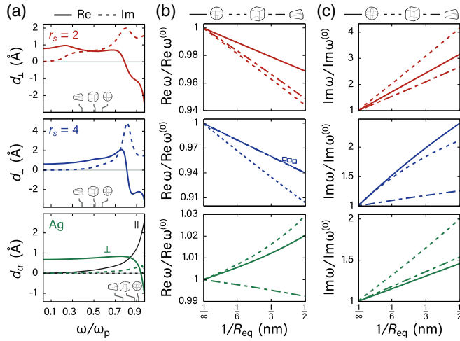
FIG. 3. The role of material, shape, and scale in the spectral properties of plasmonic nanostructures. (a) The spectral dependence of d_{\perp} for HEGs ( r_s = 2 and 4 ) and Ag ( d_{\parallel} in black). Ag is normalized by its screened plasma frequency \hbar\omega_p = 3.81 eV. (b)–(c) The real and imaginary part of the resonance dispersion with inverse scale, indicated by equivalent spherical radius R_{\text{eq}} \equiv (\frac{3}{4\pi} \times \text{volume})^{1/3} , for spheres, cubes ( a/b = 5 ), and triangles ( a/b = 3 ) for the materials considered in (a) with matching color code (HEGs; Drude decay \gamma^{(0)} = \omega_p/50 ). The classical resonance position \text{Re } \omega^{(0)} of the geometries are indicated in (a) by line-connected symbols. TDDFT calculations by Weick et al. [65] of jellium Na nanospheres ( r_s = 3.93 ) are shown in (b) by square markers.
