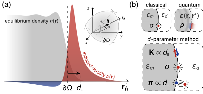
FIG. 1. Surface features in quantum plasmonics. (a) Schematic of equilibrium and induced densities, n(\mathbf{r}) and \rho(\mathbf{r}) , (distinct scales) plotted along a coordinate line, \mathbf{r}_{\hat{n}} , normal to an \hat{n} -oriented surface \partial\Omega which delimits the ionic boundary of a metallic domain \Omega , see inset. Both n(\mathbf{r}) and \rho(\mathbf{r}) may extend beyond \partial\Omega ; d_{\perp} is the centroid of \rho(\mathbf{r}) . (b) The leading-order differences between classical [local response, \epsilon_m, d_{\perp} ] and quantum accounts [nonlocal response, \epsilon(\mathbf{r}, \mathbf{r}') ; induced density \rho(\mathbb{R}^3) ] of the plasmonic response of a surface may be bridged by introducing nonclassical contributions due to surface dipole and current densities, \boldsymbol{\pi}(\mathbf{r}) and \mathbf{K}(\mathbf{r}) , proportional to the Feibelman parameters d_{\perp} and d_{\parallel} , respectively, which originate from a dipole expansion of \rho(\mathbf{r}) .
