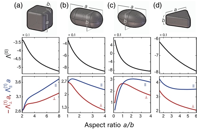
FIG. 2. Aspect ratio dependence, a/b , of the shape factors, \Lambda^{(0)} , -\Lambda_{\perp}^{(1)}a , and \Lambda_{\parallel}^{(1)}a (the latter two normalized by the length L = a ) for four canonical geometries: (a) cubes of side a and edge- and corner-rounding 2b , (b) cylindrical pills of length a , diameter b , and butt-rounding b , (c) spheroids with principal axis a and b , and (d) equilateral triangles of height b , side a , and edge- and corner-rounding \approx 0.165a . A dipole mode is considered in all cases; its induced dipole is along a in (a)–(c) and along the triangle altitude in (d). Rounding is intramural and of cylindrical and spherical kind with inscribed diameters equaling the specified rounding value.
