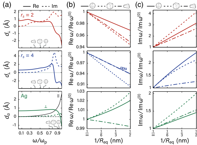
FIG. 3. The role of material, shape, and scale in the spectral properties of plasmonic nanostructures. (a) The spectral dependence of d_{\perp} for HEGs ( r_s = 2 and 4) and Ag ( d_{\parallel} in black). Ag is normalized by its screened plasma frequency \hbar\omega_p = 3.81 eV. (b)–(c) The real and imaginary part of the resonance dispersion with inverse scale, indicated by equivalent spherical radius R_{\text{eq}} \equiv (\frac{3}{4\pi} \times \text{volume})^{1/3} , for spheres, cubes ( a/b = 5 ), and triangles ( a/b = 3 ) for the materials considered in (a) with matching color code (HEGs; Drude decay \gamma^{(0)} = \omega_p/50 ). The classical resonance position \text{Re } \omega^{(0)} of the geometries are indicated in (a) by line-connected symbols. TDDFT calculations by Weick et al. [65] of jellium Na nanospheres ( r_s = 3.93 ) are shown in (b) by square markers.
