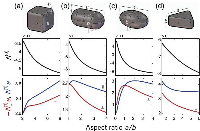
FIG. 2. Aspect ratio dependence, a/b , of the shape factors, \Lambda^{(0)} , -\Lambda_\perp^{(1)}a , and \Lambda_\parallel^{(1)}a (the latter two normalized by the length L = a ) for four canonical geometries: (a) cubes of side a and edge- and corner-rounding 2b , (b) cylindrical pills of length a , diameter b , and butt-rounding b , (c) spheroids with principal axis a and b , and (d) equilateral triangles of height b , side a , and edge- and corner-rounding \approx 0.165a . A dipole mode is considered in all cases; its induced dipole is along a in (a)–(c) and along the triangle altitude in (d). Rounding is intramural and of cylindrical and spherical kind with inscribed diameters equaling the specified rounding value.
