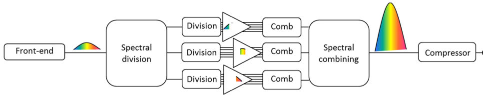
Fig. 3. Schematic of a possible pulse synthesis implementation in a CAN laser system.
