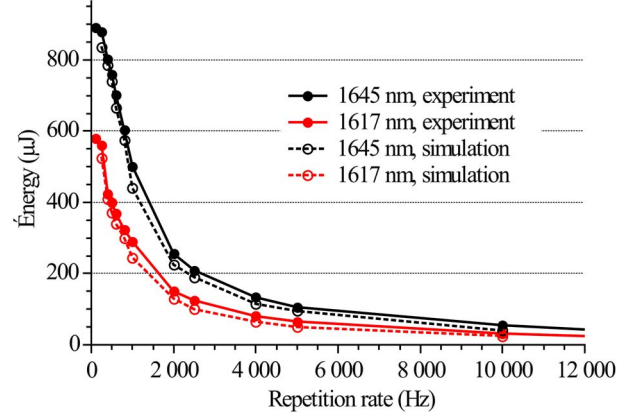
Fig. 8. Experimental (plain) and simulated (dashed) energy in AQS operation at 1645 nm (black) and 1617 nm (red).
