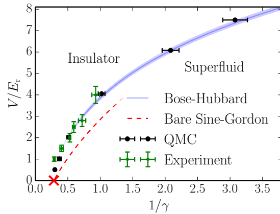
Figure 3. (Color online) Phase diagram in the g - V plane at commensurability ( na = 1 ). The black and green points, both with errorbars) are the Monte Carlo and experimental results, respectively. The blue line is the BH prediction using exact Wannier functions and the critical value (J/U)_c = 0.297 \pm 0.01 (the shaded area corresponds to this error bar). The red cross indicates the critical interaction strength g_c such that K(g_c) = 2 in the Lieb-Liniger model. Along the whole transition line the effective Luttinger parameter remains K = 2 . The red line is the result of the bare sine-Gordon theory [26].
