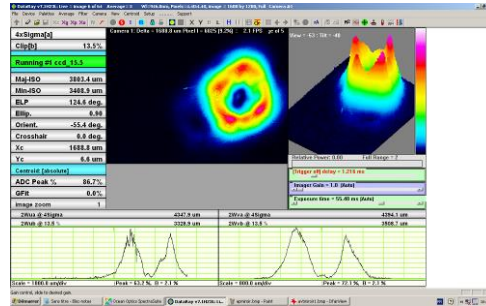
e. I_p = 8.8A ; P_p = 120W ; P_{out} = 86W
