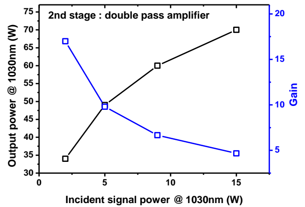
Fig 4b. Gain of the Yb:YAG SCF amplifier versus signal input power.
