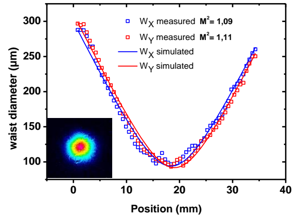
Fig 2d. M^2 measurement for the two axes.
