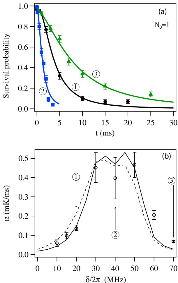
FIGURE 2: (a) Survival probability P_1(t) of a single atom in the dipole trap, measured for various detunings of the excitation light \delta/2\pi = \{20; 40; 70\} MHz (circles, squares and triangles, respectively). The trap depth is U = h \times 36 \text{ MHz} = k_B \times 1.8 \text{ mK} and the saturation parameter is s = 0.5 . Solid lines show fits of the data to a heating model (see text). The initial temperature of the single atom is T_0 = 200 \mu\text{K} . Error bars are statistical. (b) Heating rate \alpha (circles) deduced from the fits of the survival probability, versus \delta/2\pi (error bars are from the fit); the solid and dashed lines are solutions of the rate equation model described in the text, with no free parameter, for T_0 = 200 \mu\text{K} and T_0 = 300 \mu\text{K} respectively. Data labeled 1, 2 and 3 are extracted from the loss curves shown in (a).
