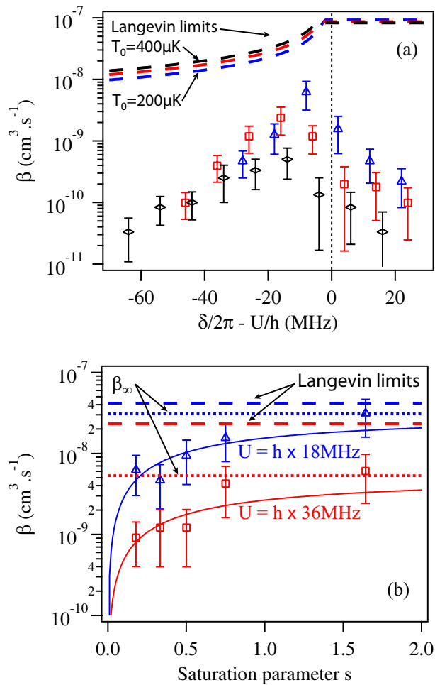
FIGURE 4: Two-body loss rate versus (a) the light-shifted detuning \delta/2\pi - U/h , and (b) the saturation parameter s of the excitation light. Triangles, squares and lozenges correspond respectively to trap depths U/h = (18; 36; 54) MHz, initial peak atomic densities n_0 = (2.7; 4.3; 5.1) \times 10^{12} \text{ cm}^{-3} and initial temperatures T_0 = (200; 300; 400) \mu\text{K} . The average initial atom number is \langle N_0 \rangle \simeq 3 for all the data. Error bars are from the fits. The dashed lines are the Langevin limits \beta_L associated to each set of parameters (U, T_0) (see text). In (a), the saturation parameter is s = 0.5 . In (b), the detuning of the excitation is \delta/2\pi = 10 MHz. The solid lines are fits of the data to a \beta_\infty s/(1+s) model (with \beta_\infty the only free parameter). The dotted lines indicate the asymptotical value \beta_\infty in each case.
