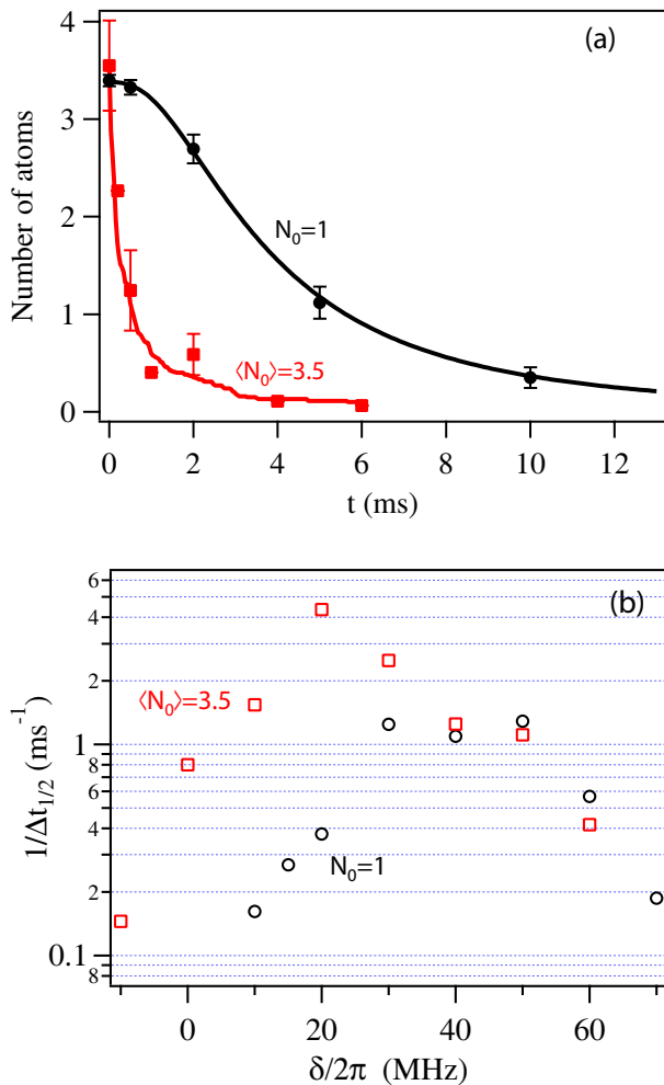
FIGURE 3: (a) Average number of atoms \langle N(t) \rangle remaining in the dipole trap after excitation by a light pulse with duration t . Squares : the initial number of atoms in the trap is \langle N_0 \rangle = 3.5 ; the solid line is a fit to a Monte-Carlo simulation (see text), with a heating rate \alpha = 0.21 mK/ms and a two-body loss rate \beta' = 1.2 (at.ms) ^{-1} . Circles : single-atom measurements rescaled to N_0 = 3.5 ; the solid line is a fit to the radiative heating model. Error bars are statistical. Parameters of the experiments : U/h = 36 MHz, \delta/2\pi = 20 MHz, s = 0.5 . (b) Inverse of the half-lifetime in the cases \langle N_0 \rangle = 3.5 (squares) and N_0 = 1 (circles) versus the detuning of the excitation light.
