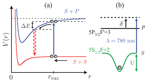
FIGURE 1: (a) Light-assisted atom loss by radiative escape. Atoms in the S state interact through the Van der Waals potential V(r) = -C_6/r^6 while atoms in the S and P states interact through the dipole-dipole attractive potential V(r) = -C_3/r^3 . (b) Levels involved in the experiment. The excitation laser detuning \delta is measured with respect to the free space transition.
