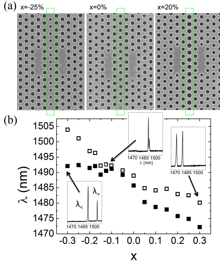
Fig. 7. (a) SEM images of coupled L3 cavities on a suspended membrane with barrier engineering, for three hole sizes in the barrier. (b) Measured resonant wavelengths of splitted modes ( \lambda_{<} : filled squares, and \lambda_{>} : empty squares) as a function of the barrier modification. Inset: PL spectra showing mode splitting. Pump power is \sim 30\mu W . Target fabrication parameters are those of Fig. 4.
