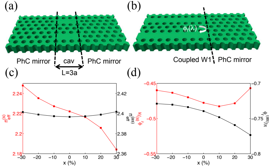
Fig. 2. Building-up the Fabry-Perot model. (a) An optical defect is composed by a “free propagation” cavity region of length L = 3a surrounded by two PhC mirrors; the boundary between the cavity region and the mirror is given by the dashed lines. (b) Phase of the modal reflection [\phi_r(\lambda)] of the Bloch modes of two coupled W1 waveguides on a PhC mirror. (c) Effective index of symmetric (red) and anti-symmetric (black) Bloch modes. The values of the effective index are taken at the resonance wavelengths of the cavities. (d) Idem as in (c) for the reflectivity phases at resonance.
