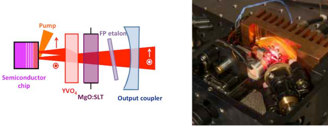
Figure 2. (left) scheme of the laser setup; (right) photograph of the dual-frequency laser prototype.
