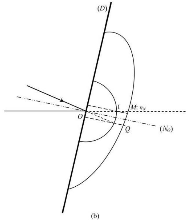
Fig. 2. Vectorial analysis of the Descartes's construction. (a) Case of a normally incident ray. (b) Effect of small tilts of (N_o) and of the incident ray. The index surfaces remain fixed, and the upper dashed line normal to (D) shows Descartes's construction when the incident ray also remains fixed (horizontal on this figure) and only \{(D), (N_o)\} is slightly tilted, leading to the term in \delta \mathbf{v} ; the translation from the upper to the lower dashed line is due to \delta \mathbf{r} , and shows the change in Descartes's construction when the incident ray is slightly rotated.
