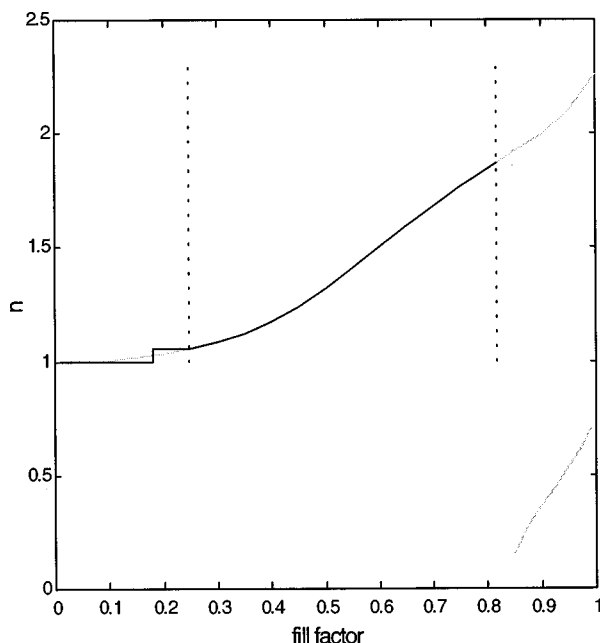
Fig. 11. Calibration curve used for the design of blazed binary diffractive components as a function of the fill factors. Thin curves: n values of all the propagating modes supported by a bi-periodic structure composed of a 405-nm-period array of square pillars engraved in a 2.23-refractive-index material. The upper curve ( n varying from 1 to 2.23) corresponds to the fundamental mode or effective index. Vertical dotted lines: limits imposed by fabrication constraints for \Delta_1 = 100 nm and \Delta_2 = 75 nm. Thick curve: modified calibration curve.
