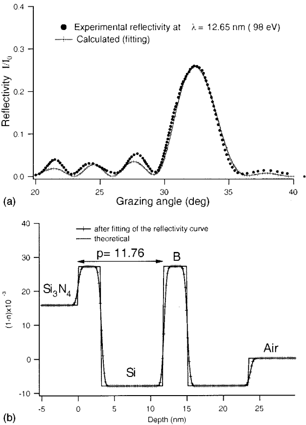
FIG. 9. (a) Measured and fitted reflectivity of B/Si multilayers versus grazing angle at \lambda=12.6 \text{ nm} . (b) Parameters of fits and simulated optical index profile at \lambda=12.6 \text{ nm} . The continuous line curve corresponds to theoretical parameters: bulk indices and perfect interfaces, the other curve is calculated from resulting parameters of the fit given in Table II.
