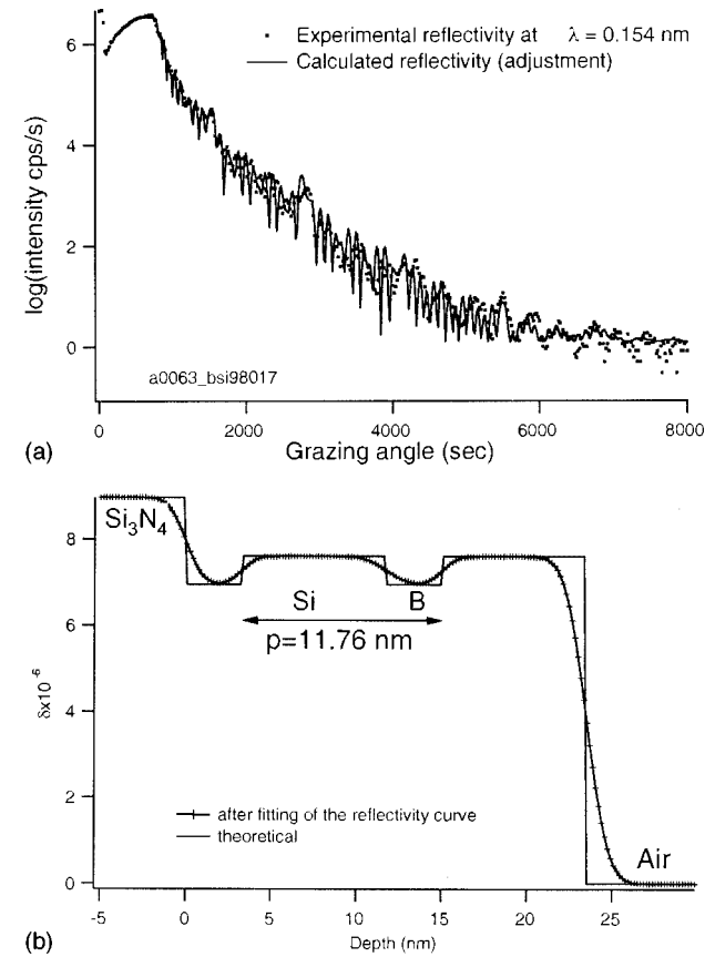
FIG. 8. (a) Measured and fitted reflectivity of B/Si multilayers versus grazing angle at \lambda=0.154 \text{ nm} . (b) Simulated optical index profile at \lambda=0.154 \text{ nm} . The continuous line curve corresponds to theoretical parameters: bulk indices and perfect interfaces, the other curve is calculated from resulting parameters of the fit given in Table I.
