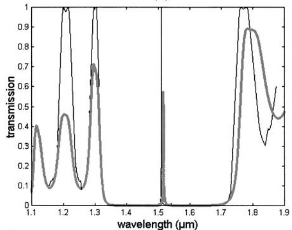
Fig. 10. Air-bridge microcavity: (a) Dimensions of the photonic bandgap air-bridge microcavity. Each square hole has a 250-nm side. (b) Computational box and absorbers. (c) Theoretical transmission of the photonic bandgap air-bridge microcavity. Thicker curve, the present method; thin curve, the finite-element modal method with perfectly conducting walls.
