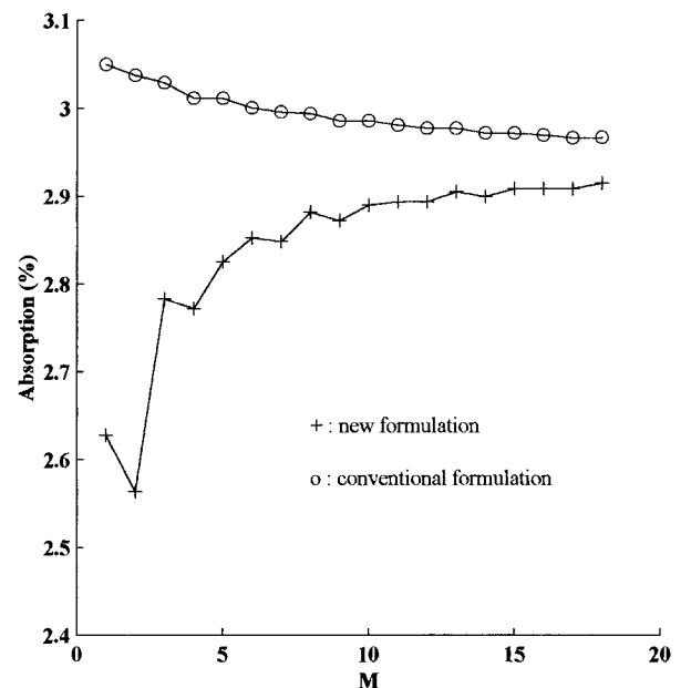
Fig. 6. Same as Fig. 4, except that h = 0.005\lambda .
