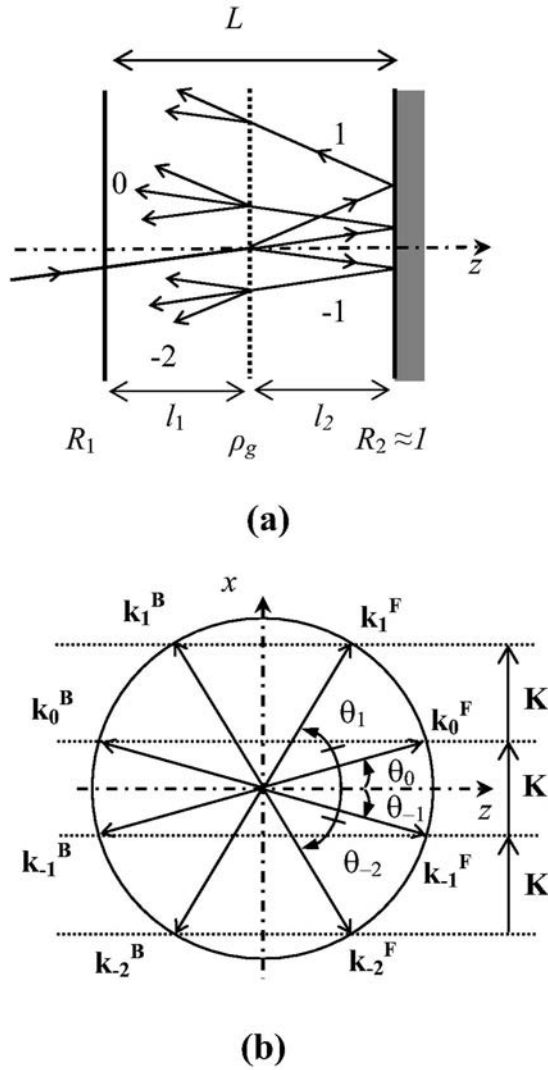
Fig. 1. (a) Setup of the thin grating inside the Fabry-Perot resonator and (b) the wave vectors of all considered diffraction orders.
