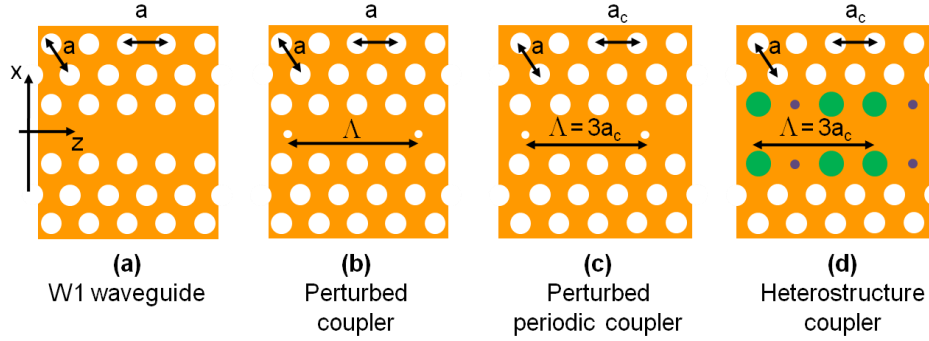
Fig. 1. Successive steps of the design process. The objective is to realize a periodic diffractive element compatible with the PhC periodicity and able to couple/extract light in/from the PhCW shown in (a). The waveguide is formed by removing one row of holes in a triangular lattice (period a = 430 \text{ nm} ) of air holes (radius r = 110 \text{ nm} ) etched into an InP membrane (refractive index n = 3.16 and thickness h = 265 \text{ nm} ). (b) Adding a periodic perturbation (super-period \Lambda ) to the W1 waveguide creates in general an aperiodic coupler because both periods a and \Lambda are not commensurate. (c) A periodic coupler is obtained by increasing the longitudinal period of the PhC, a_c = a + 30 \text{ nm} = 460 \text{ nm} , in order to render \Lambda and the new period a_c commensurate, \Lambda = 3a_c . (d) We have chosen to keep the holes position unchanged and to create the periodic perturbation by increasing and decreasing the radius of the two inner rows of holes ( r_c = r \pm \Delta r ). We obtain a heterostructure coupler with a super-period \Lambda = 3a_c .
