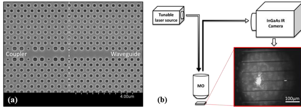
Fig. 3. (a) SEM picture of the interface between the W1 waveguide (on the right of the dashed-dotted white line) and the heterostructure coupler (on the left of the dashed-dotted white line). (b) Simplified description of the transmission measurement setup. The red framed picture shows different parallel waveguides (horizontal dark lines) with light being coupled into the central one. The large bright spot on the left is the incident spot reflected by the input coupler and the weak elongated spot on the right correspond to the output coupler and shows where the light is extracted from the waveguide.
