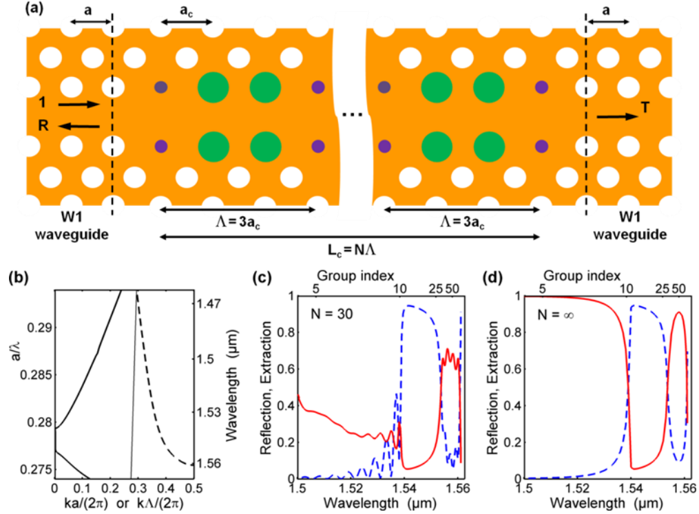
Fig. 2. Coupler performance. (a) The heterostructure coupler shown in Fig. 1(d) with \Delta r = 35 nm is inserted between two semi-infinite W1 waveguides. The coupler has a finite length L_c = N\Lambda and its performance can be quantified by the reflection R , the transmission T and the extraction efficiency O = 1 - R - T . (b) Dispersion curves of the guided Bloch mode of the W1 waveguide (dashed line) and of the leaky Bloch mode of the coupler (solid line). The latter lies above the light line (thin solid line). The guided Bloch mode of the W1 waveguide is used as the incident mode in the scattering problem in (a). Its cutoff wavelength where n_g \rightarrow \infty is \lambda_g \approx 1.561 \mu\text{m} . (c) Reflection R (dashed blue line) and extraction O (solid red line) as a function of the wavelength for N = 30 . (d) Same quantities for a semi-infinite coupler ( N = \infty and O = 1 - R since T = 0 ). Large extraction efficiencies can be obtained around n_g = 50 .
