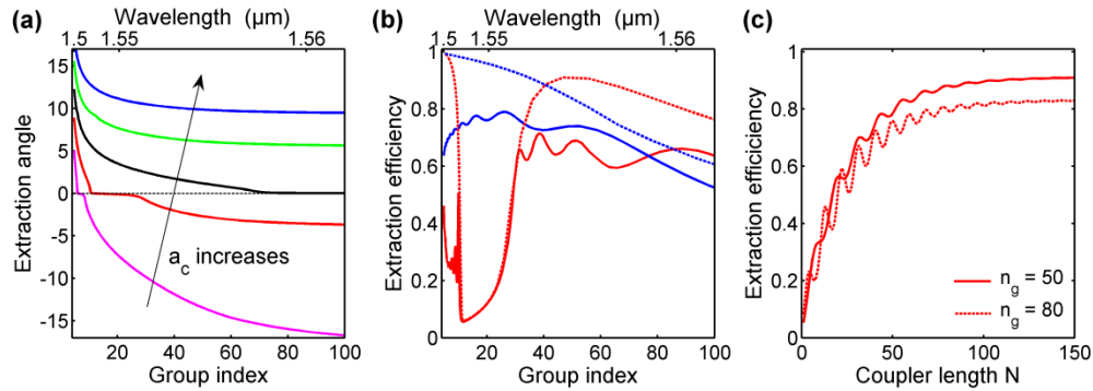
Fig. 5. Performance of the coupler for different values of the longitudinal period a_c . The other geometrical parameters of the system are the same as in Fig. 1(d) with \Delta r = 35 nm. (a) Extraction angle \theta for a_c = 450, 460, 470, 480 and 490 nm (magenta, red, black, green and blue curves respectively). (b) Extraction efficiency O = 1 - R - T for a_c = 460 nm (red) and a_c = 490 nm (blue). Solid and dashed curves correspond to N = 30 and N = \infty (semi-infinite coupler). (c) Extraction efficiency as a function of the coupler length for a_c = 460 nm. N is the number of super-periods in the coupler, L_c = N\Lambda , see Fig. 2(a). Solid and dashed curves correspond to n_g = 50 and n_g = 80 .
