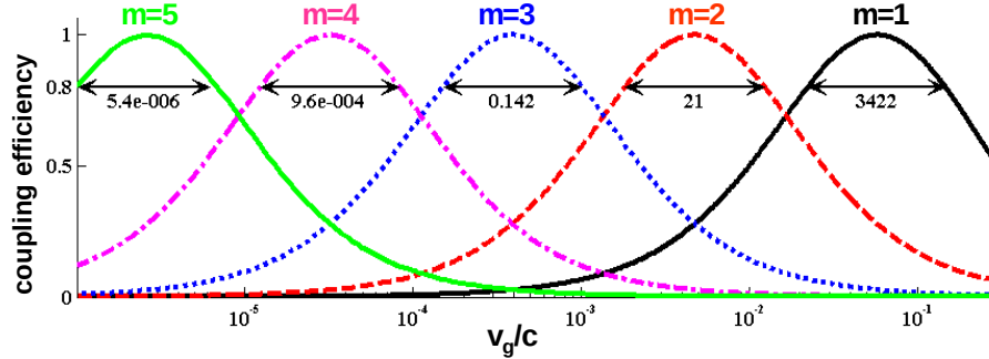
Fig. 3. Coupling efficiency into the slow-mode of a periodic stack ( n_H , n_L ) as a function of the group velocity (log scale) of the slow mode. Different injectors are considered. They are all composed of Bragg mirrors ( n_H , n_L ) with an increasing number of repeated pairs, m=1, \dots, 5 . The results are obtained in the vicinity of the valence band edge of the periodic stack. The horizontal arrows indicate the bandwidths in GHz of the different injectors for T=0.8 (-1dB).
