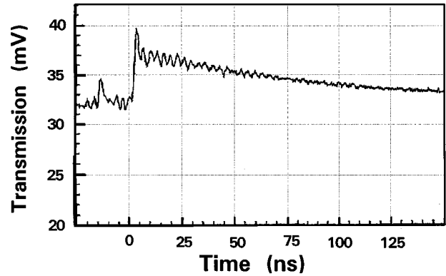
FIG. 5. Measured nanosecond transmission transient for VO 2 probed with a 633 nm cw HeNe laser.
