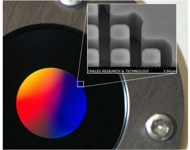
Fig. 2. (Color online) Subwavelength BPM and scanning electron microphotograph showing the border between the inner and the outer ring. To synthesize the desired effective index and thus the desired phase in the inner zone, the geometry of the pillars is controlled properly and manufactured through optical lithography and inductively coupled plasma etching.
