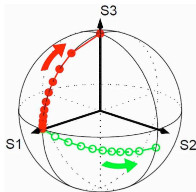
Fig. 3. (Color online) Representation of \vec{s}_{opt} (●) and \vec{t}_{opt} (○) for different values of \gamma from 0 to 0.1 on the Poincaré sphere. Arrows indicate increasing values of \gamma .
