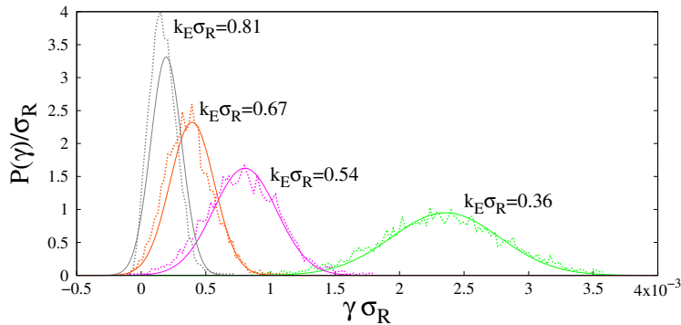
Figure 3. (Color online) Probability distributions of the Lyapunov exponents obtained by transfer matrix calculations (dotted lines) with the disorder parameters of Fig. 2, V_R > 0 (space step of \Delta z = 0.1\sigma_R and total system size of L_{\text{tot}} = 13333\sigma_R with random initial conditions), and various energies (indicated on the figure). The solid lines are the corresponding theoretical distributions (10).
