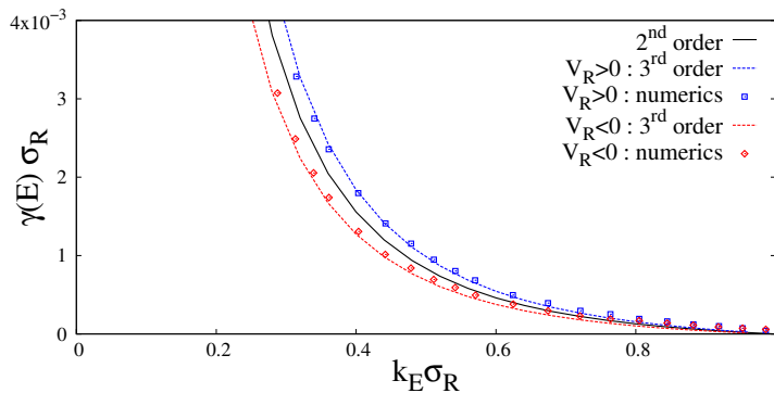
Figure 2. (Color online) Lyapunov exponent for both blue- and red-detuned speckles with the standard correlation function (2) and V_R = \pm 0.01625(\hbar^2/m\sigma_R^2) . Shown are the numerical results extracted from a transfer matrix method (space step of \Delta z = 0.1\sigma_R and total system size of L_{\text{tot}} = 411775\sigma_R with random initial conditions) averaged over 5000 disorder realizations (blue squares: V_R > 0 , red diamonds: V_R < 0 ), and analytical results obtained from the phase formalism up to order 2 (solid black line) and up to order 3 (dotted blue and red lines).
