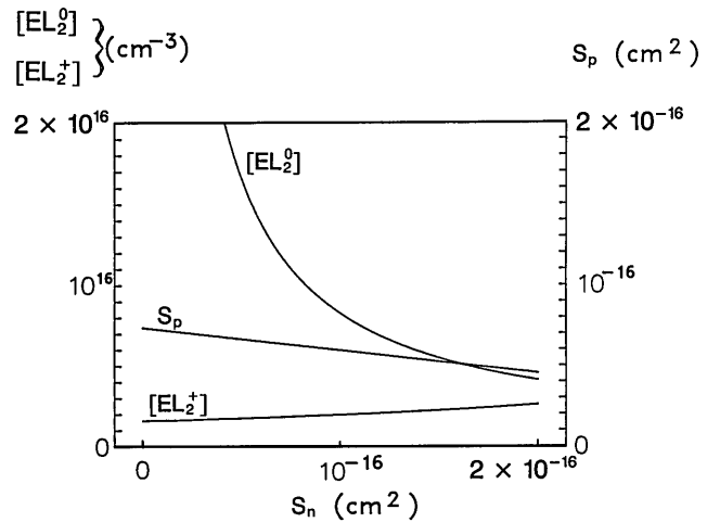
Fig. 5. Variation of S_p , [\text{EL}_2^0] , [\text{EL}_2^+] as a function of S_n .
