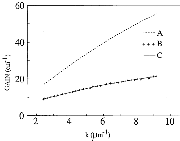
Fig. 1. Curve A, theoretical gain expected from a Fe 2+ /Fe 3+ level coupled with both conduction and valence bands with \xi = 1 ( \alpha_n \ll \alpha_p ) and k_0^2 = 500 \mu\text{m}^{-2} ( [\text{Fe}^{2+}] = 10^{-16} \text{cm}^{-3} \ll [\text{Fe}^{3+}] ). Curve B, experimental gain. Curve C, theoretical gain with contribution of the Fe 2+* level considered.
