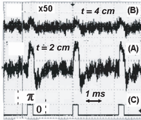
Fig. 2. Normalised one shot ac -signal obtained with thicknesses t = 2 cm (A) and 128 averaged (B) with t = 4 cm ( \times 50 ) chicken breast and P = 0.1 MPa. Trace (C) shows the phase modulation of the US ( \omega_{mod} = 305 Hz, cyclic ratio = 1/8 ).
