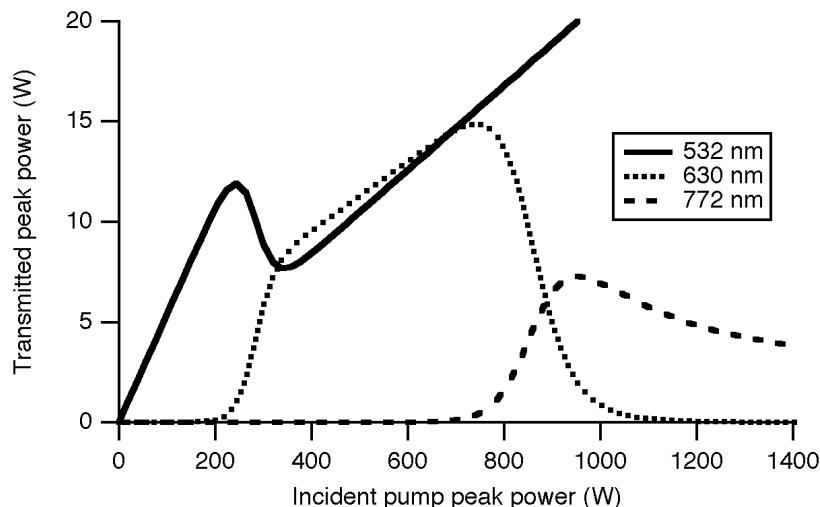
Fig. 5. Theoretical dependence of the pump and Stokes lines intensities.
