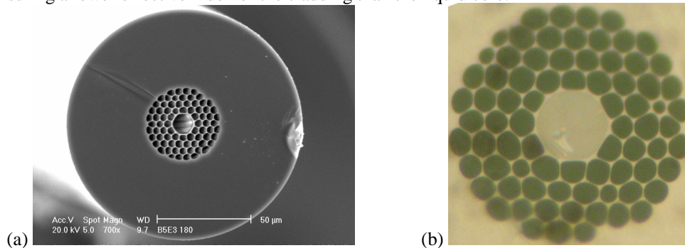
Fig. 1. (a) SEM image of used fiber, (b) Optical microscope image of the end of the fiber filled with water and illuminated from above. The peripheral holes were closed on the side where liquid was inserted, and the fiber is observed on the cleaved other side. Only the central hole is filled with the liquid.
