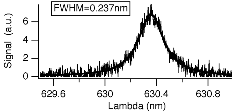
Fig. 3. Spectrum of first Stokes lines at 630nm. The bold line represents an adjustment with a Lorentzian profile, with the given width.
