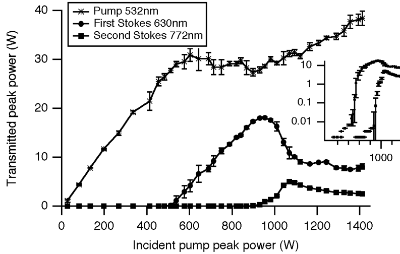
Fig. 4. Intensity dependence of the transmitted pump, and Stokes lines as a function of the incident pump beam intensity. The insert shows the Stokes intensities on a log scale allowing a precise determination of the threshold.
