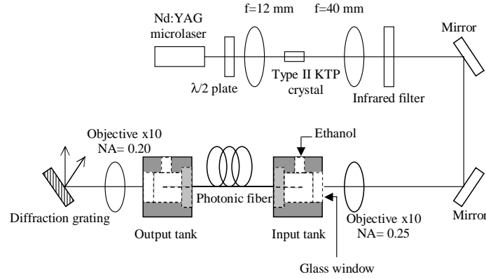
Fig. 2. Experimental set-up for the measurement of Stimulated Raman Scattering in liquid core photonic crystal fiber.
