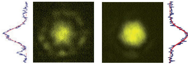
Figure 8. (Color online) Near-field patterns of the pump (left) and of the first Stokes line (right).
