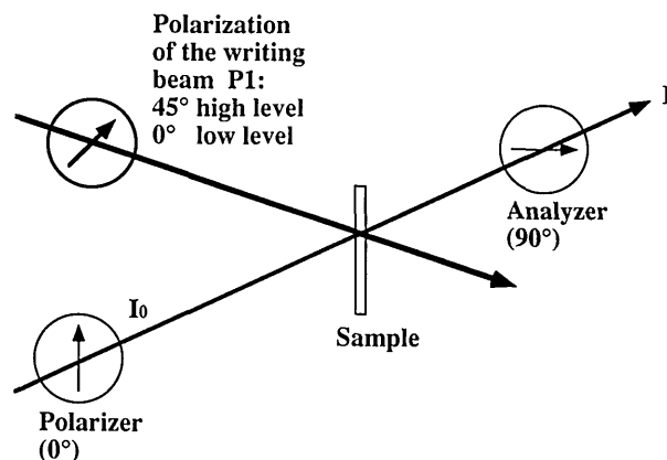
Fig. 1. Experimental setup. I_0 , input energy; I , output energy. Sample has thickness e , birefringence \Delta n = n_{ex} - n_{or} .
