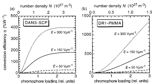
Fig. 10. Calculated normalized second-harmonic conversion efficiency \eta as a function of chromophore density for DANS-SCP and DR1-PMMA for three (external) poling fields E . The relative units are defined such that unity corresponds to the actual loading of the chromophores in the polymers used for the measurements. The corresponding chromophore number densities N are indicated on the top axes. The waveguide was assumed to be 1 cm long; the other parameters are identical to those in Fig. 9.
