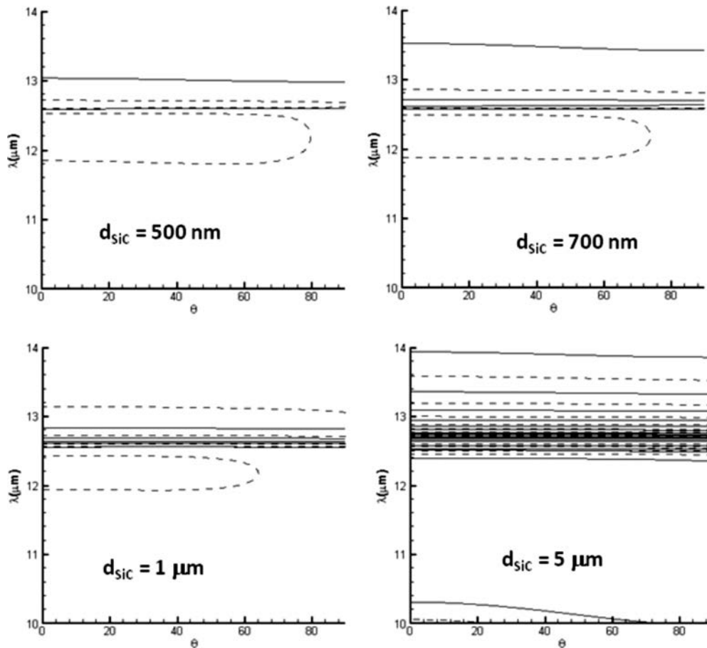
FIG. 7. Dispersion relations of propagative resonant modes in TE polarization with d_{\text{Ge}}=735 nm. In dotted line is plotted the real part of the equation \mathcal{T}_{11} = 0 while in solid line is represented its imaginary part.
