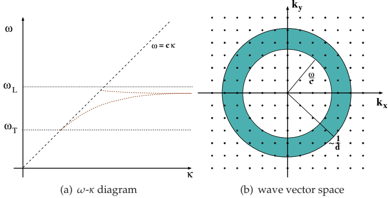
Fig. 4. Sketch of the surface phonon polariton modes for a given distance d . relation (Kliwer and Fuchs (1974))
