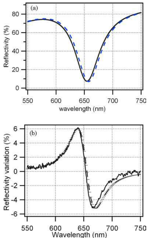
Fig. 2. (Color online) (a) Plasmon spectrum before (solid curve) and after (dashed curve) the functionalization of the probe. (b) Reflectivity variation after the functionalization of the probe molecule on the surface. The solid and the dashed lines are the experimental and the theoretical responses, respectively.
