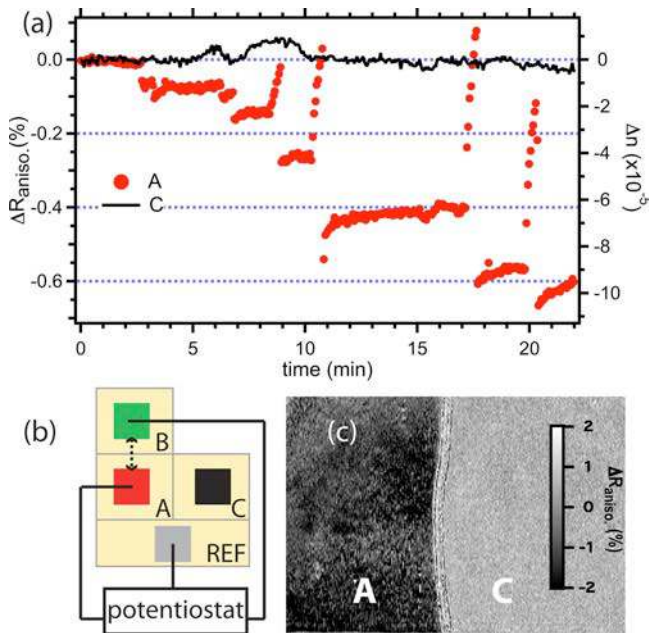
Fig. 3. (Color online) (a) Dynamical P-SPRI signal of a SAM-supported hemimembrane system. Dots, anisotropic response of electrode A. Line, response of electrode C (control). (b) Diagram of the biochip areas. (c) Image of the differential SPR anisotropy observed.
