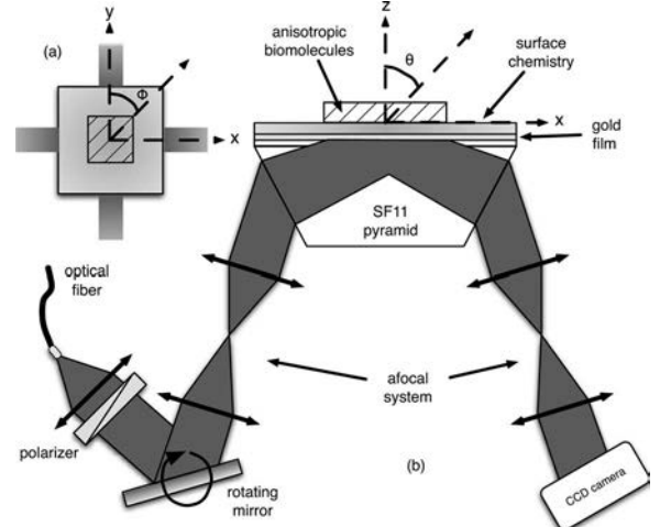
Fig. 1. Schematic representation of the P-SPRI system. (a) Top view. (b) Side view.
