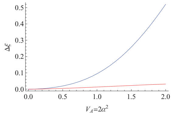
FIG. 2. (Color online) Equivalent excess noise \Delta\xi due to the non-Gaussian modulation as a function of the variance of modulation V_A . Upper curve refers to the four-state protocol, lower curve to the eight-dimensional protocol. By definition, a protocol with a Gaussian modulation does not display any equivalent excess noise. An excess noise of one unit of shot noise corresponds to an entanglement-breaking channel, therefore no security is possible with such a level of noise. This figure clearly shows that the eight-dimensional protocol outperforms significantly the four-state protocol.
