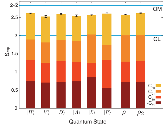
FIG. 3 (color). Experimental violation of the state-independent temporal Bell inequality (7). The classical limit is indicated by CL and the maximal achievable quantum value by QM. The first six bars correspond to pure signal states, the remaining two to mixed inputs, as explained in the main text. The latter were obtained by switching the signal state between states |D\rangle and |A\rangle while measurements were performed. The relative integration for |D\rangle and |A\rangle were chosen according to the target purity of 0.5 for \rho_1 and 0.75 for \rho_2 . The mixed states were verified via single-qubit tomography.
