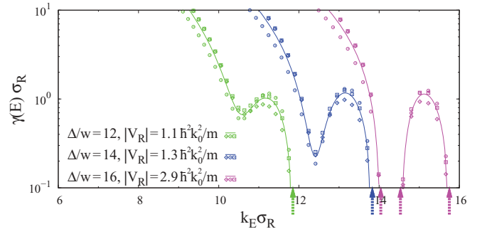
FIG. 4. (Color online) Lyapunov exponents along the transport eigenaxes ( x : diamonds; y : dots; z : squares) and their geometric averages (solid lines) versus energy in a 3D speckle potential created by two Gaussian beams (waist w and separation \Delta ) for various parameters (indicated in the figure). The arrows indicate the mobility edges. We recall that \sigma_R = \lambda_0 l/\pi w .
