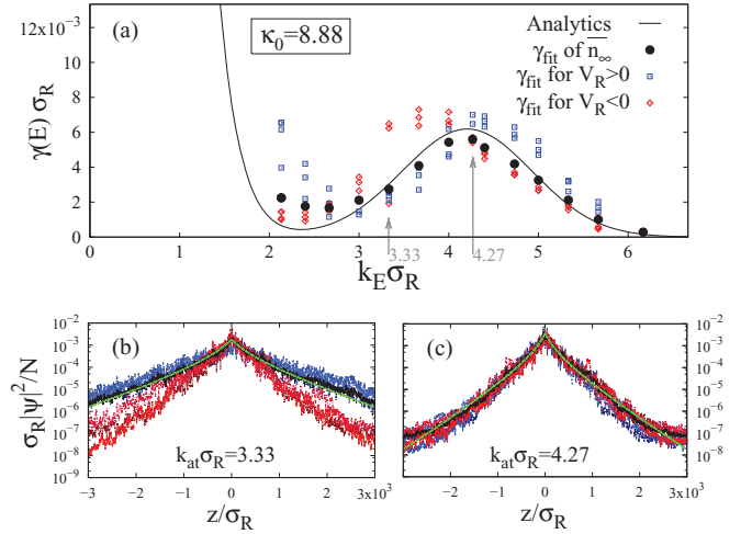
FIG. 2. (Color online) Anderson localization in 1D speckle potentials with the autocorrelation function (3), \kappa_0 = 8.88 , and V_R = \pm 0.72(\hbar^2/m\sigma_R^2) . (a) Lyapunov exponent versus particle energy as obtained from Eq. (2) (solid black line) and from fits of Eq. (4) to the numerical data (points). (b), (c) Stationary density profiles obtained numerically using the initial state (5) with p_w \sigma_R / \hbar = 0.24 and two different values of p_{at} . The figures show the results for six realizations of the disorder [three with V_R > 0 (blue upper data) and three with V_R < 0 (red lower data)], the averaged density profile (black central data), and the fits of P_\infty(z) to the latter (green solid line). The extracted values of \gamma_{fit} for each realization and for the averaged profile are reported in (a). The figure shows a significant increase of the Lyapunov exponent in the energy window such that 2.3 \lesssim k_E \sigma_R \lesssim 4.2 .
