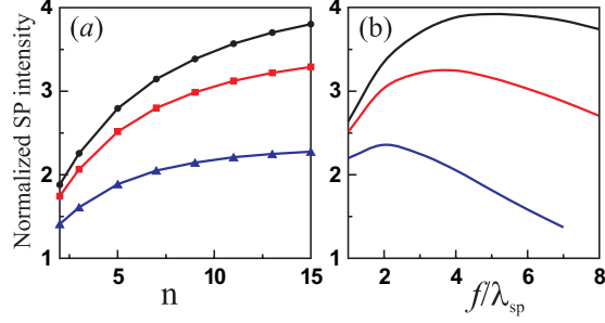
Fig. 4. (a) Normalized intensity of surface plasmon field diffracted by a Fresnel lens made of an array of N = 2n + 1 slits with a focal distance f = 3\lambda_{sp} versus n . (b) Normalized intensity of the surface plasmon field diffracted by a Fresnel lens made of a nonperiodical array of N = 2n + 1 slits, n = 13 , as a function of the focal distance f . The calculation has been performed for the different surface plasmon wavelengths: \lambda_{sp} = 435 nm (black circles (a), black curve (b)), 400 nm (red squares (a), red curve (b)), 375 nm (blue triangles (a) and blue curve (b)). The lines in figure (a) are for eyes guidance.
