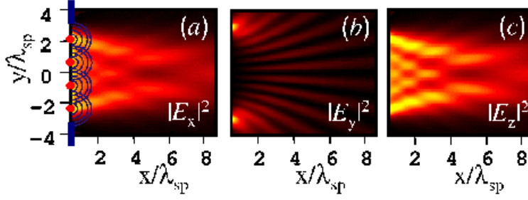
Fig. 1. Diffraction pattern of a slit with width w = 6\lambda_{sp} illuminated from the left by a homogeneous surface plasmon at normal incidence. \lambda_{sp} = 400 nm. The intensity is normalized by the intensity of the z-component of the incident surface plasmon field at x=0 . Black is zero intensity. Yellow indicates the maximum intensity and corresponds to 0.25 in (a) 0.01 in (b), and 1.2 in (c).
