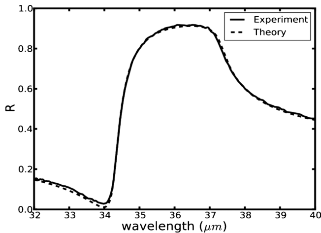
FIG. 2. Reflectivity of a GaAs flat surface ( \theta_i = 15^\circ ).
