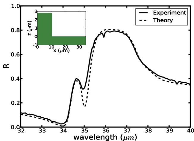
FIG. 3. (Color online) Reflectivity of a GaAs grating and simulated geometry in the inset ( \theta_i = 15^\circ ).
