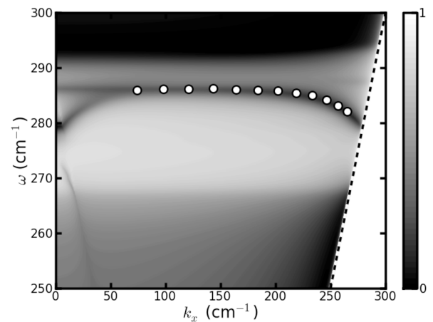
FIG. 4. Reflectivity map calculated for a GaAs grating of 35 \mu\text{m} period with a filling factor of 0.3 and a height of 2.8 \mu\text{m} . White is for high reflectivity, while black is for low reflectivity. White filled circles indicate the position of measured reflectivity dips.
