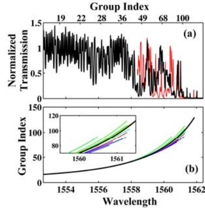
Fig. 2. Experimental data collected for the twenty PhCWs. (a) Spectra of two different waveguide instances (black and red curves). n_g dependence (top axis) is deduced from interferometric measurements (b) n_g(\lambda) curves recorded for every waveguide. The large spreading at large n_g 's (inset) results from disorder-induced fluctuations that smear the sharp cutoff at v_g = 0 . The thick-black curve represents the ensemble-averaged curve used to relate the actual wavelength to an averaged group index.
