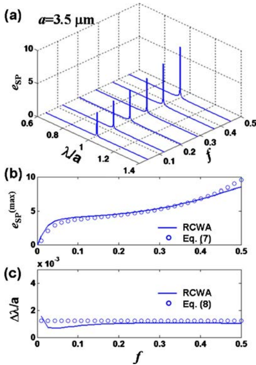
Fig. 6. (Color online) Influence of the slit width. (a) Normalized SPP-excitation rate as a function of the wavelength for a=3.5 \mu\text{m} and for various slit widths w ( f=w/a ). The results are obtained with the RCWA for normal incidence ( e_{\text{SP}}^+ = e_{\text{SP}}^- = e_{\text{SP}} ). (b) Peak value of e_{\text{SP}} . (c) Peak width \Delta\lambda . In (b) and (c), the RCWA data and analytical data are shown with solid curves and circles, respectively.
