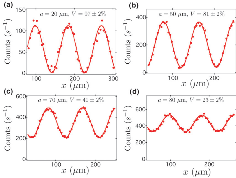
Figure 4. Photocounts recorded on detector P_1 while translating the grating G along the x -axis, for different widths a of the transmitting slits: (a) a = 20 \mu\text{m} , (b) 50 \mu\text{m} , (c) 70 \mu\text{m} and (d) 80 \mu\text{m} . Identical results are recorded on detector P_2 . The grating is translated by 4\text{-}\mu\text{m} steps and each point is recorded with 3\text{-s} acquisition time. A constant averaged background due to detector dark count rate (about 180 \text{ counts s}^{-1} ) has been subtracted from the data. The visibility is evaluated using a fit by a cosine function shown as a solid line.
